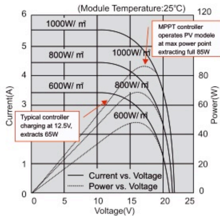
Figure 1 Current, Power vs. Voltage Characteristics
